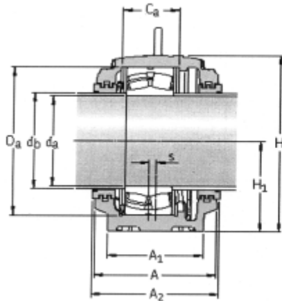
Labyrinth seals. TS design
