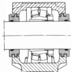
Type TS Housing with labyrinth seals
