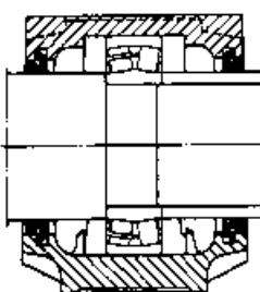
Type TA Housing with V-ring seals
