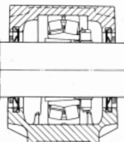
Type TA Housing with V-ring seals
