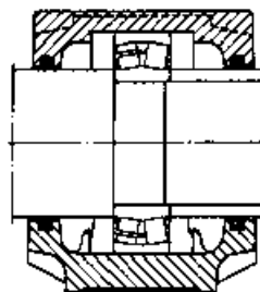
Type TC Housing with felt seals
