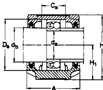
Type TG Housing with double-lip seals
