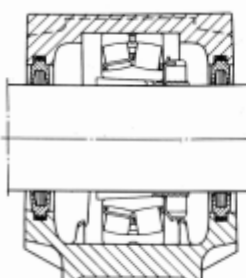
Type TC Housing with felt seals
