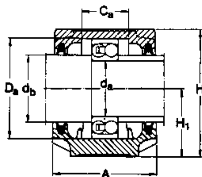
Type TG Housing with double-lips seals
