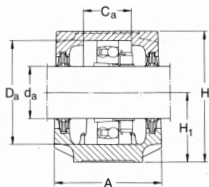
Type TG Housing with double-lips seals
